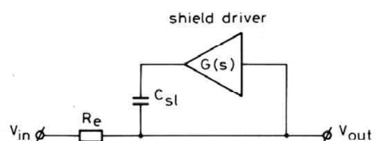
Fig. 7 Simplified diagram of the guarding circuit shown in Fig. 6
