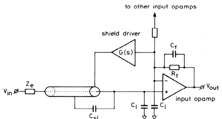
Fig. 6 The feedback loop formed by a guarding circuit. The loop is closed by the capacitance between the shield and the inner core C_{sl} . The operational amplifier is the input stage of an instrumentation amplifier
