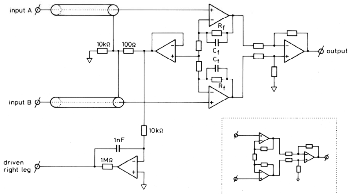
Fig. 3 Biomedical instrumentation amplifier equipped with guarding and driven right leg circuits, based on the three operational amplifier instrumentation amplifier (see inlay)
